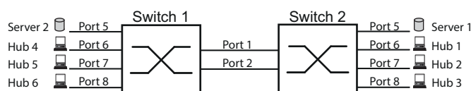
Abb. 42: Link Aggregation Switch-zu-Switch-Netz
